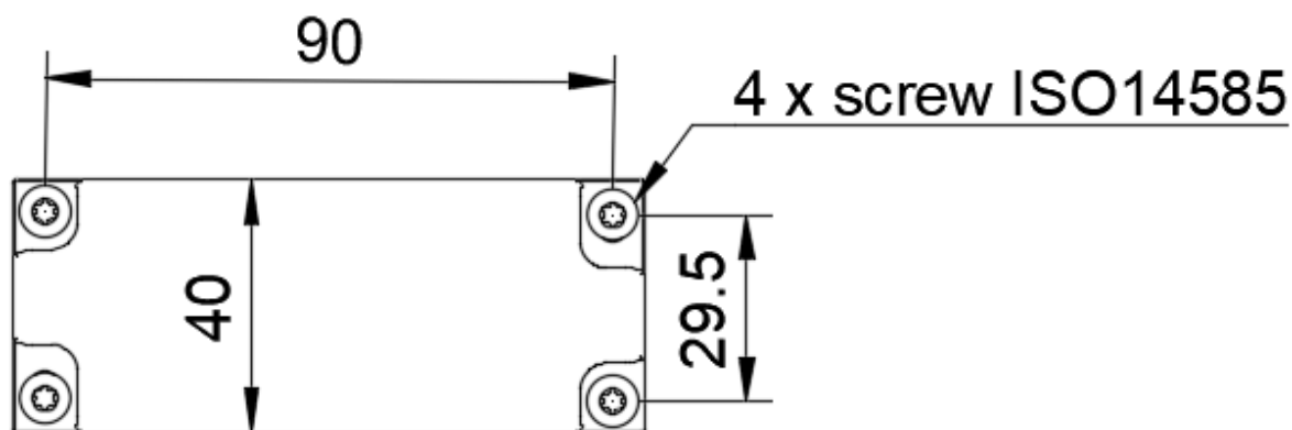
Top view, with screw
