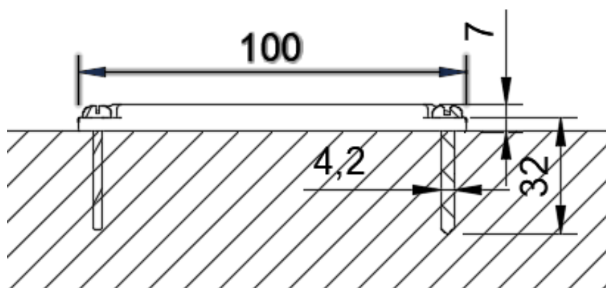
Front view, mounted on surface
